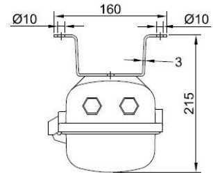
High ceiling mounting with clamp TYPE "V"
