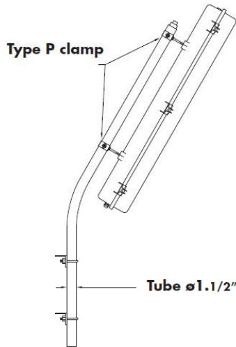
Standard pole mounting
