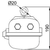
Pendant mounting with eyebolt TYPE "O"
