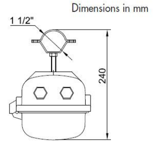
Mounting using 1.1/2" metal clamps TYPE "P"
