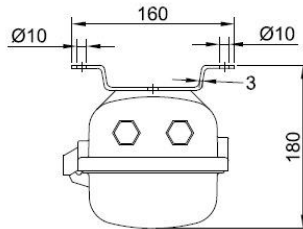
Low ceiling mounting with clamp TYPE "U"
